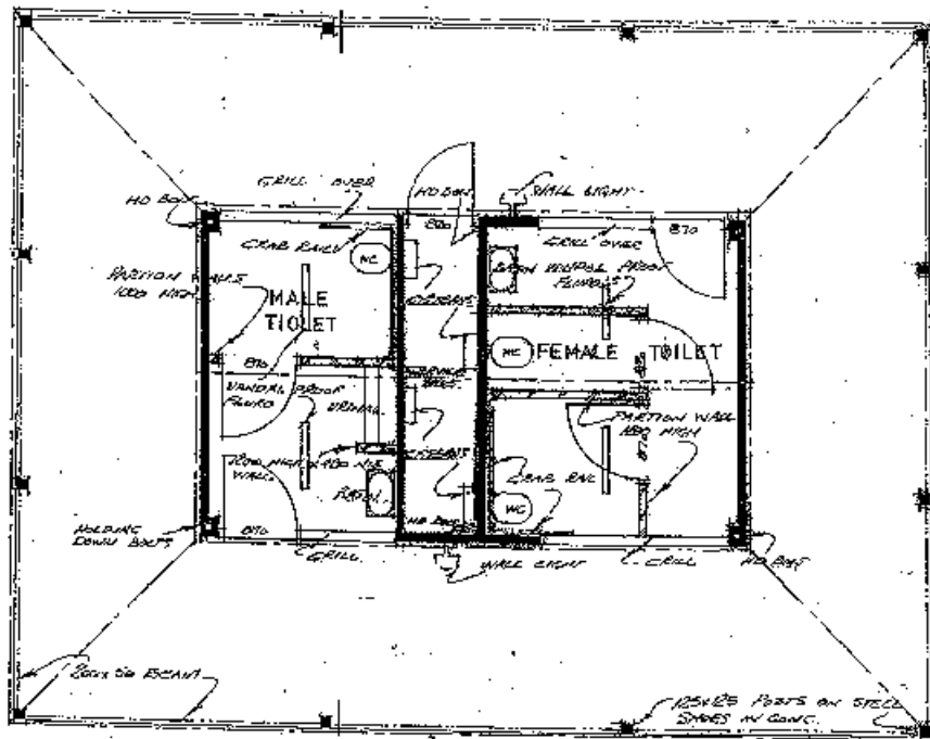
PROPOSED FLOOR PLAN AND LAYOUT OF CONVENTIONAL TYPE PUBLIC TOILETS
