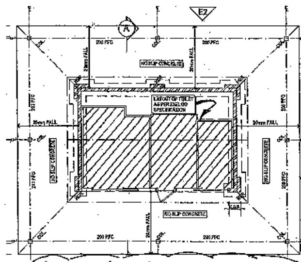
PROPOSED ROOF STRUCTURE TO HOUSE TWIN SELF CLEANING TOILET MODULE AS DETAILED ABOVE.
