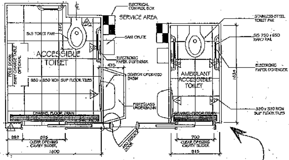
FLOOR PLAN LAYOUT TYPICAL LAYOUT OF TWIN SELF CLEANING TOILET MODULE UNIT
